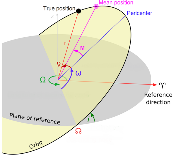
Figure 1.11: Illustration of the orbital parameters and configuration, with the observer's direction z .
