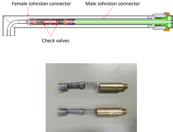
Figure 3.12: Top : Layout of the Johnstone coupling. Note the check valves highlighted in pink. Bottom : Photograph of the feed line's check valve (top) and the manifold's check valve with orifices (bottom).
