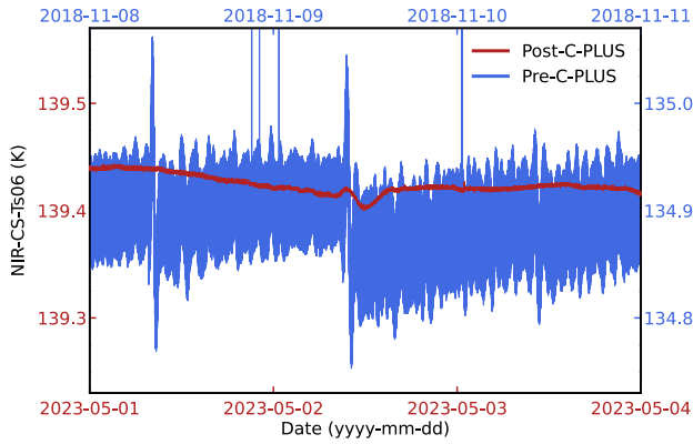
Figure 3.8: Temperature variability over 3-day intervals at the heat exchanger attached to the radiation shield (NIR-CS-Ts06).
