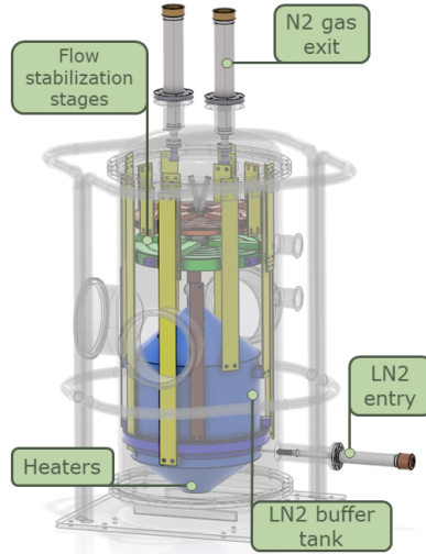
Figure 3.7: Preliminary CAD design of a new N2GPU-Evo.
