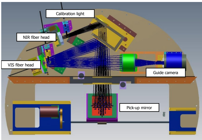
Figure 1.13: Opto-mechanical layout of the CARMENES FE.
