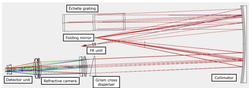
Figure 1.15: CARMENES NIR optical layout with the identified elements.
