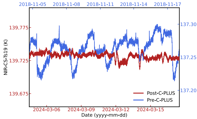
Figure 3.13: Temperature measured by the NIR-CS-Ts19 sensor.
