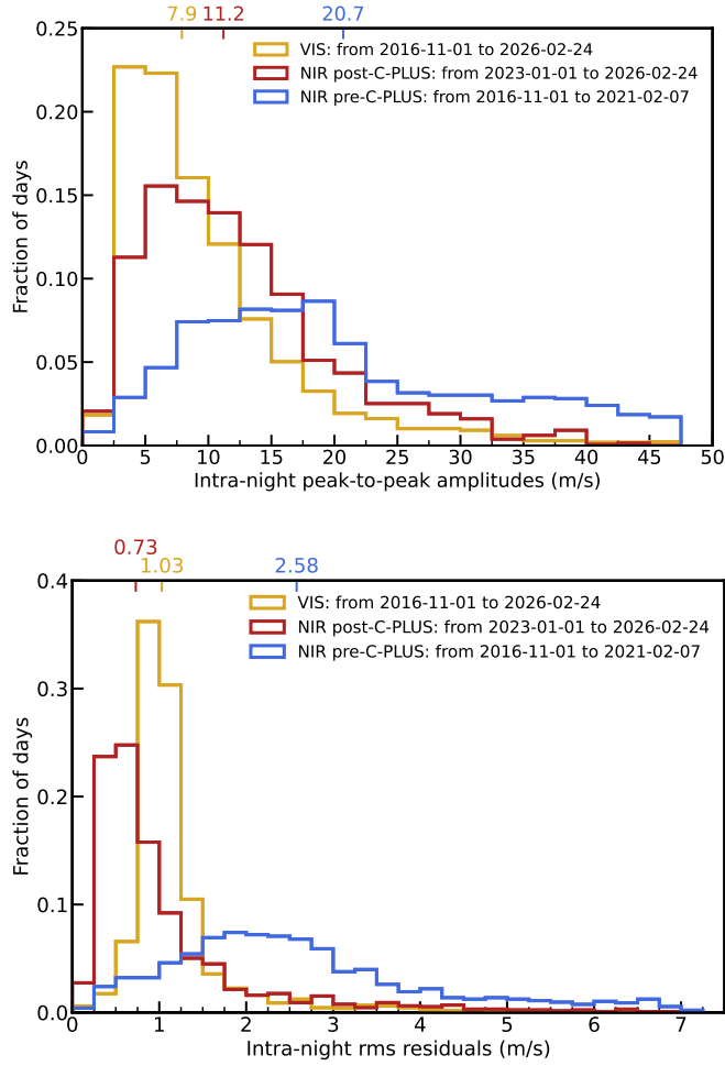
Figure 3.17: Top: Histogram of the peak-to-peak RV variation from FP calibrations. Bottom: Histogram of the \text{rms}_{\text{res}} after subtracting a quadratic fit. The median values are indicated on the top axis.
