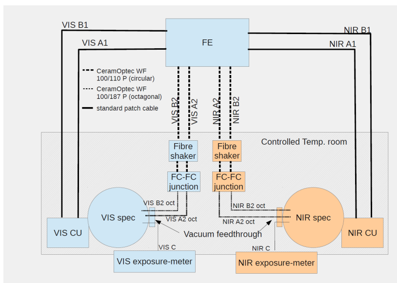
Figure 1.14: Layout of the fibers connecting the FE, CU, and spectrographs of CARMENES.
