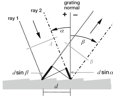
Figure 1.12: Sketch of the grating diffraction. Two parallel rays in phase reach the grating, with groove distance d , and incident and reflecting angles \alpha and \beta , respectively (Palmer, 2020).
