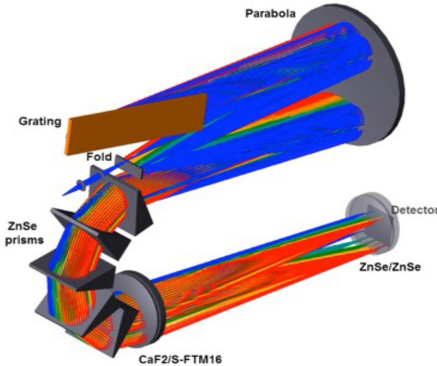
Figure 1.18: Optical layout of NIRPS spectrograph (Bouchy et al., 2025).
