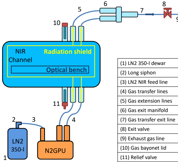
Figure 1.16: Simplified layout of the CARMENES cooling system during normal operation showing the main components, escribed in Becerril et al. (2016).
