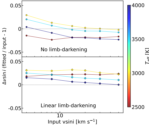
Figure 4.19: Normalized difference between input and fitted v \sin i as a function of input v \sin i and spectra's T_{\text{eff}} , without limb darkening (top panel) and with linear limb darkening (bottom panel), using NIR synthetic spectra.
