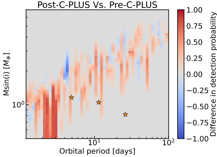
Figure 5.11: Differential detection map between post- and pre-C-PLUS RV time series (i.e. detection map of pre-C-PLUS subtracted from the post-C-PLUS one). Teegarden's b, c, and d are represented by the star markers.
