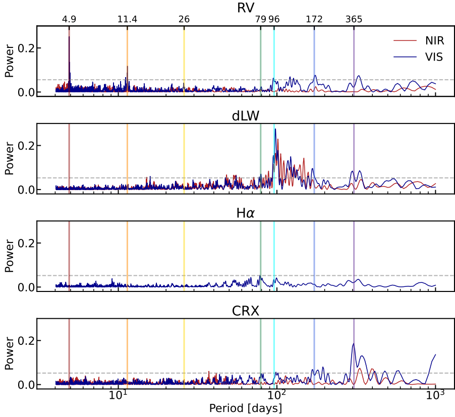
Figure 5.7: GLS periodogram of Teegarden's star of NIR and VIS RV, dLW, H\alpha , and CRX. The vertical lines represent the observed periodic signals, (i) at 4.92, 11.42, and 26.1 days for the Keplerians, (ii) 79 and 96 days for the rotational period, (iii) the 172 days signal, and the 1-year alias.
