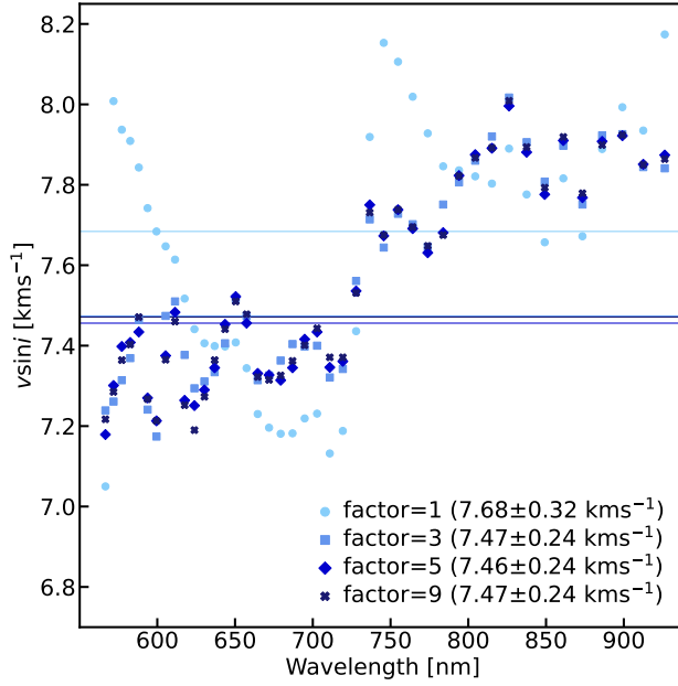
Figure 4.6: Best-fitting v \sin i values as a function of wavelength for different over-sampling factors, obtained without accounting for limb darkening in the convolution process. Horizontal lines correspond to the median values. The spectra correspond to T_{\text{eff}} = 3000 \text{ K} and a target value of v \sin i = 8 \text{ km s}^{-1} .
